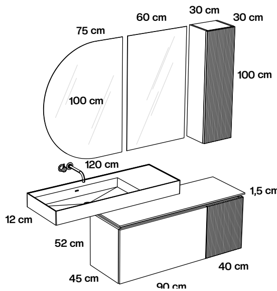
Ref. LA0852440D Módulo decorativo altura 52 cm puerta moldurada terminal derecho (Decorative module 52 cm height, lichen door and terminal right panel) 40 x 52 x 45 cm
